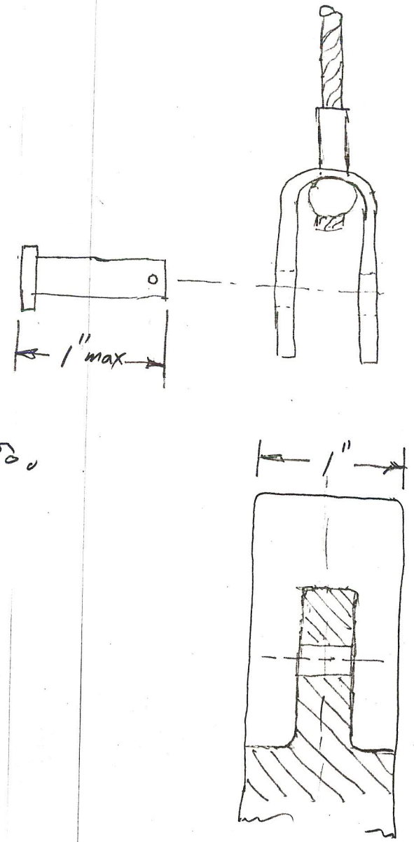
Sect. A-A
